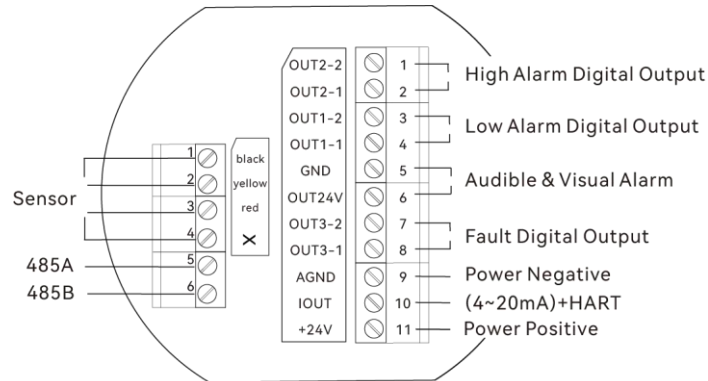
Terminal block diagram Figure 1: Wiring Terminal Diagram
